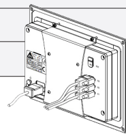
Mounting Frame (1197274-01)
